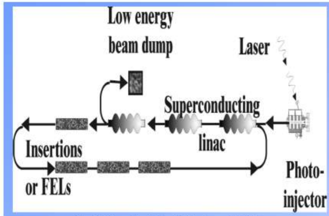
Fig. 2.12 One of traditional ERL schemes for FELs
