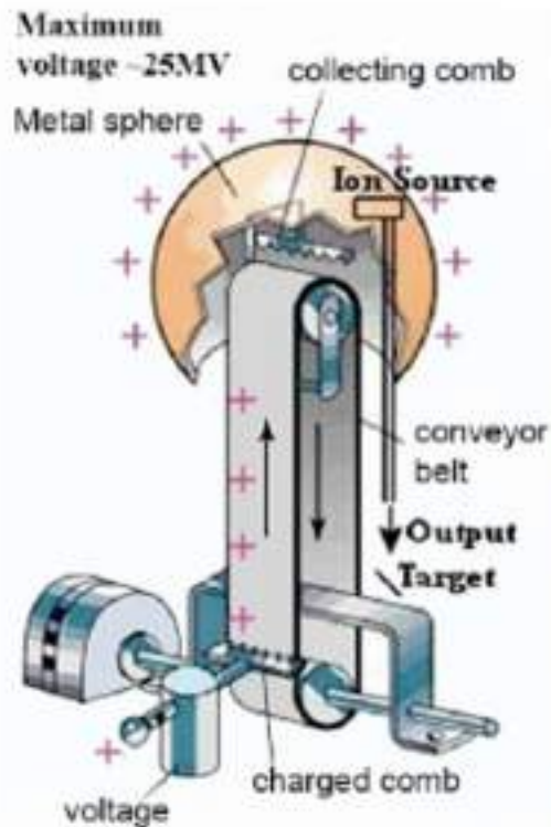
Fig. 2.4. Idea of the Van de Graaff invented an electrostatic generator and one of the biggest tandem accelerators at Daresbury (UK) with 42 m (14 stories high) 20 MV acceleration tube, placed vertically (Photo: CCLRC).
