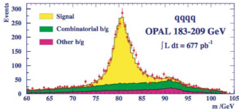
Figure 19. Reconstructed W mass distribution for all OPAL W^+W^- \rightarrow q\bar{q}q\bar{q} data from \sqrt{s} = 183 to 209 GeV. The histogram shows the SM expectation for M_W = 80.42 GeV.
