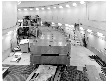
Fig. 1.2 The ZGS at Argonne, IL, USA, during construction, a 12 GeV synchrotron zero-gradient synchrotron, which used wedge focusing (field index zero). ZGS was operated over 1964-1979. First polarized beam acceleration happened at ZGS, in July 1973, to 8.5 GeV/c, up to 12 GeV/c in the following years [7,8]. Pulsed quadrupoles were used to pass through several depolarizing resonances with no significant depolarization, a method known as resonance crossing by fast “tune-jump”. Injector: protons from a 20 keV polarized source are pre-accelerated by a 750 keV Cockcroft-Walton, followed by a 50 MeV linac.
