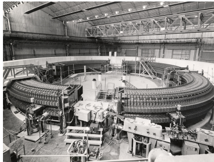
Fig. 1.1 SATURNE 1 at Saclay, France [Archives historiques CEA. Copyright CEA/Service de documentation - FAR_SA_N_xxxx], a 3 GeV, 4-periodic, 68.9 m closed orbit, weak focusing synchrotron ( n \approx 0.6 ), started operation in 1957 - plans for polarized proton beams in SATURNE 1 triggered the Froissart-Stora theory of depolarization [6,7]. Each magnet weighs 1150 tons. The four straight sections are 4 m long; injection is in the north one, from a 3.6 MeV Van de Graaff (not visible); the south section houses the extraction system; the RF cavity is in the west one; a beam detection system is located in the east one. The peak power requested from the acceleration RF system does not exceed 2 kW (a “Ham Radio” style of amplifier).
