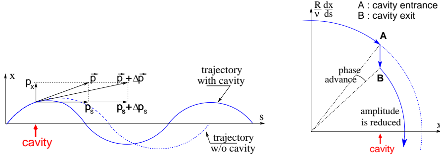
Fig. 1.6 Adiabatic damping of betatron oscillations ( \frac{\Delta p}{p} > 0 ), here from x'_{\text{in}} = p_x/p_s before the cavity, to x'_{\text{out}} = p_x/(p_s + \Delta p_s) after the cavity. In the horizontal phase space, to the right, \downarrow \Delta \left( \frac{dx}{ds} \right) if \frac{dx}{ds} > 0 , \uparrow \Delta \left( \frac{dx}{ds} \right) if \frac{dx}{ds} < 0 .
