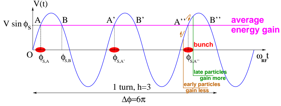
Fig. 1.7 Mechanism of phase stability, “longitudinal focussing”. Below transition, \gamma < \gamma_{tr} , \eta > 0 , acceleration occurs for a stable synchronous phase \in ]0, \pi] , at A, A', A'' in this illustration: a particle with higher energy goes around the ring quicker than synchronous particle, it arrives earlier (at \phi < \phi_{s,A} ), it will experience a lower voltage than the synchronous particle and will progress towards the latter, in energy and in phase. A particle with lower energy takes more time, it arrives later, at \phi > \phi_{s,A} , it will experience a greater voltage than the synchronous particle. Beyond transition, \gamma > \gamma_{tr} , \eta < 0 , the stable phase \in [\pi, 2\pi[ , at B, B', B'' here, with a similar stabilizing mechanism: a particle which is less energetic than the synchronous particle arrives earlier, \phi < \phi_{s,B} , and it sees a higher voltage, and inversely for a particle which is more energetic.
