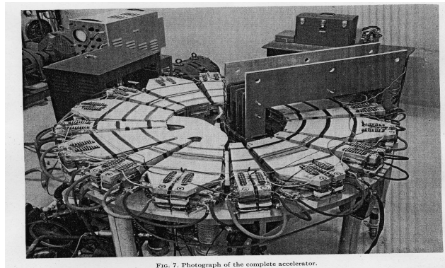
FIG. 7. Photograph of the complete accelerator.
