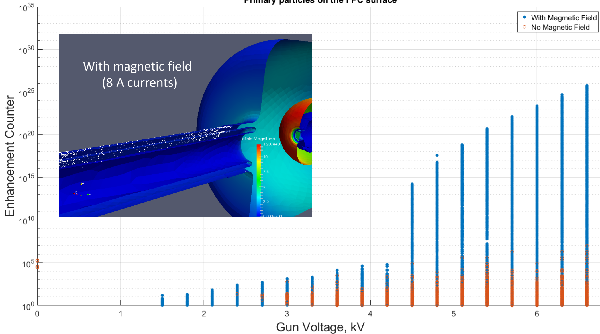
Primary particles on the FPC surface
