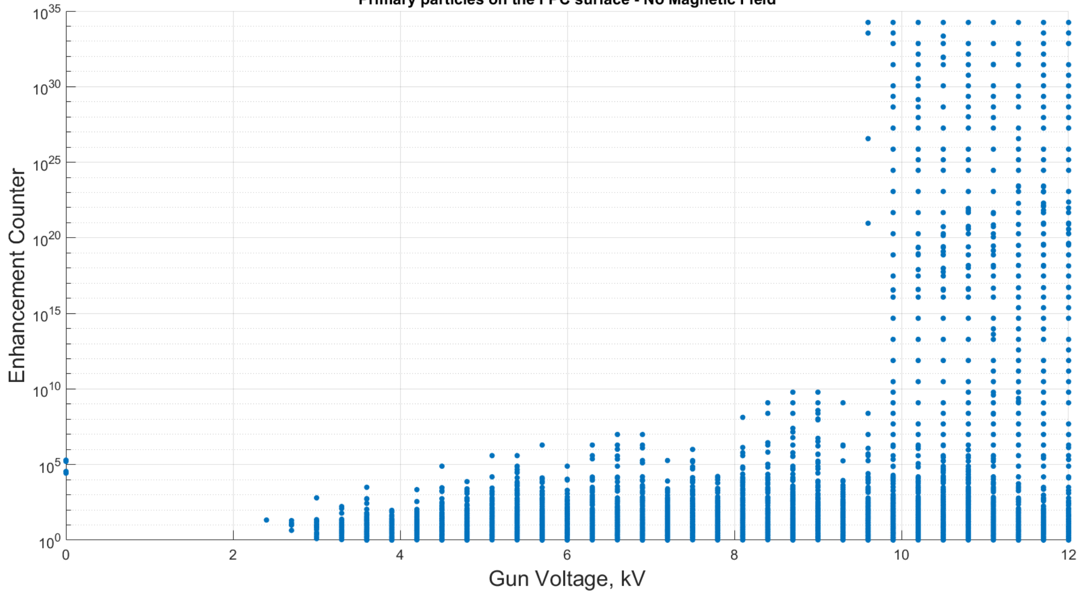
Primary particles on the FPC surface - No Magnetic Field
