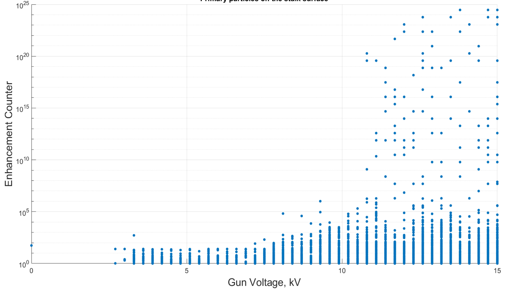
Primary particles on the stalk surface
