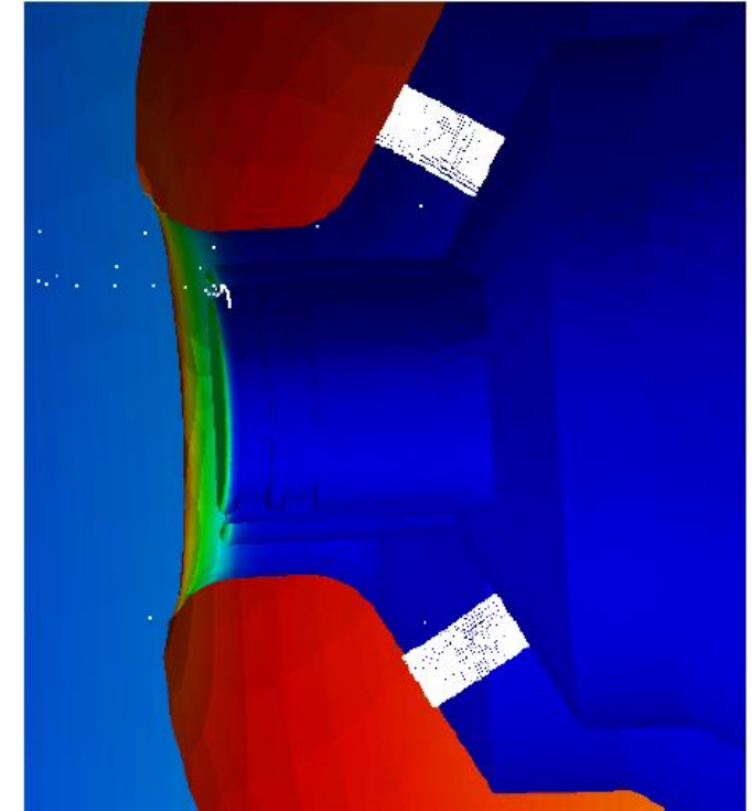
Stable trajectories at 850 kV
