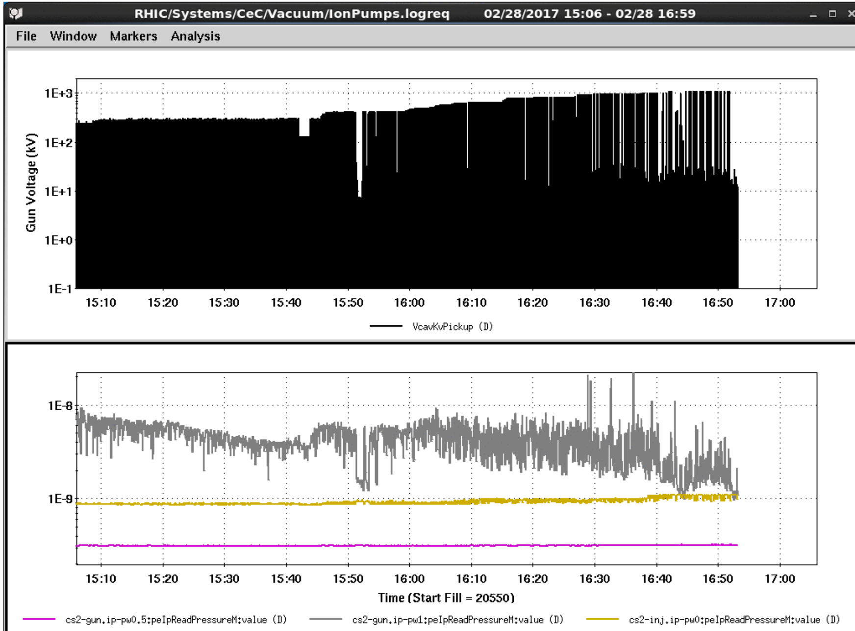
Stable trajectories at 850 kV
