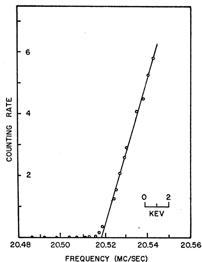
FIG. 1. Typical Li 7 (p,n)Be 7 threshold calibration.
